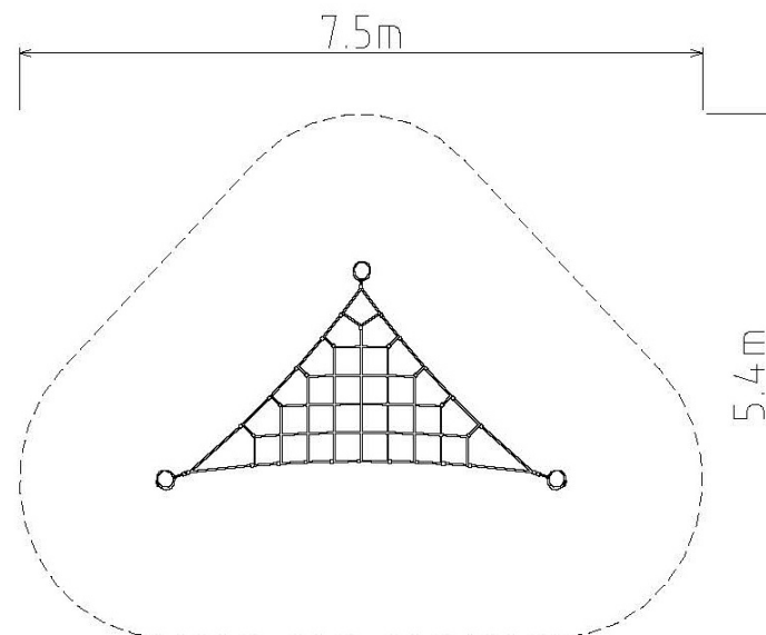
Fig. G1. Fall Zone Plan Not to scale
