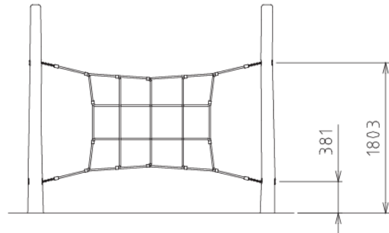
Fig. G3. Elevation Not to scale
