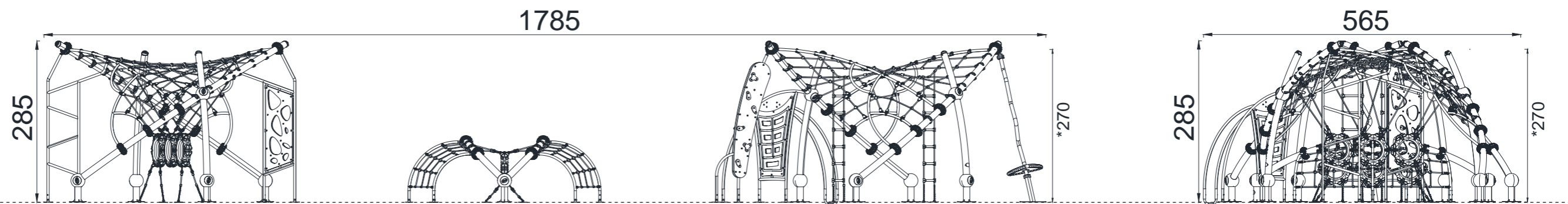
FRONT VIEW
