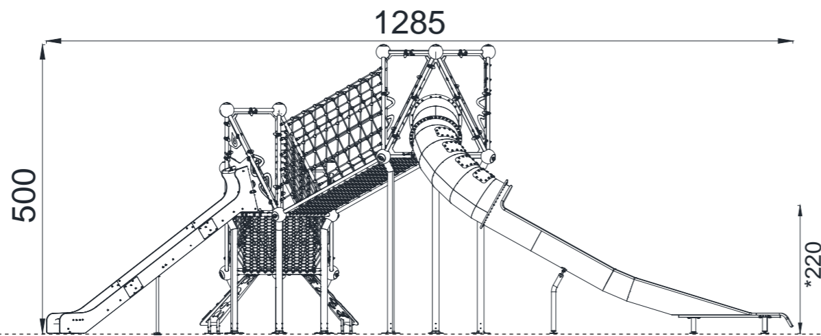
FRONT VIEW
