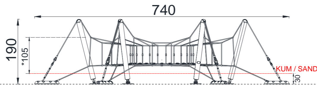
FRONT VIEW
