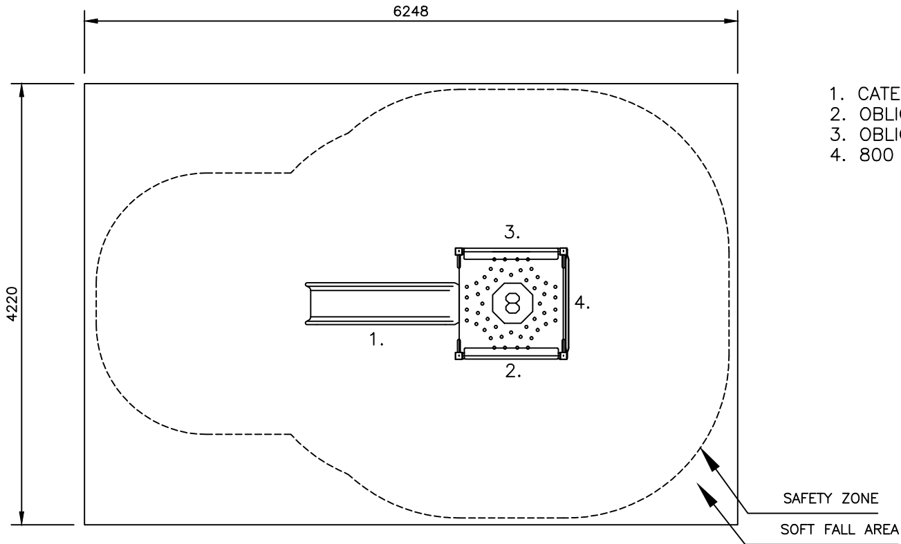
SLDP2014-800 FREESTANDING SLIDE MAX FHF: 0.8M
