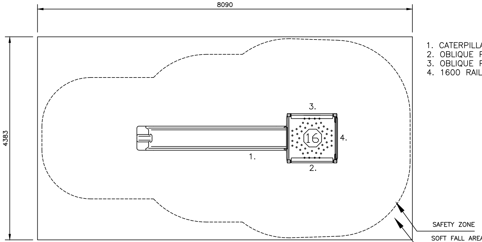
SLDP2017-1600 FREESTANDING SLIDE MAX FHF: 1.6M
