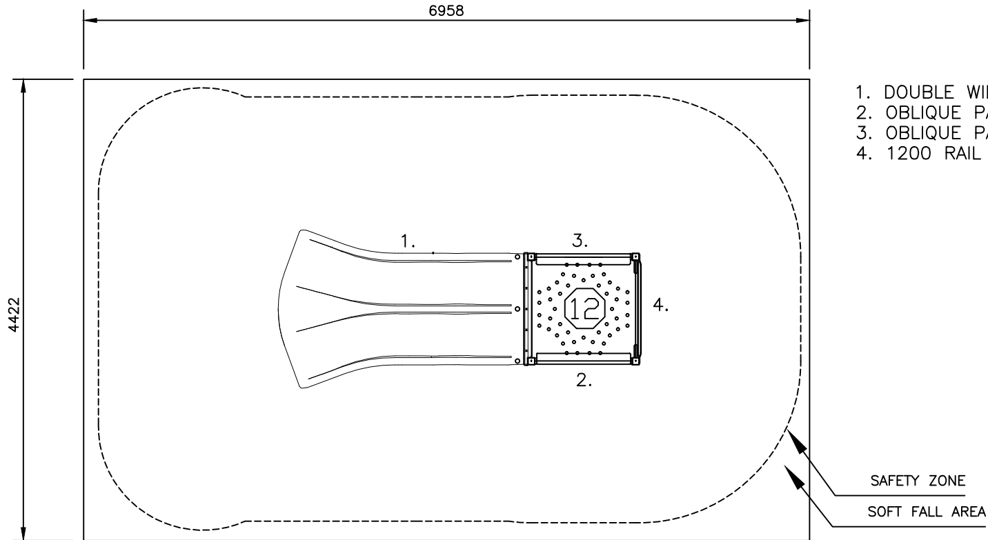
SLDP2018-1200 DOUBLE WIDE FREESTANDING SLIDE MAX FHF: 1.2M
