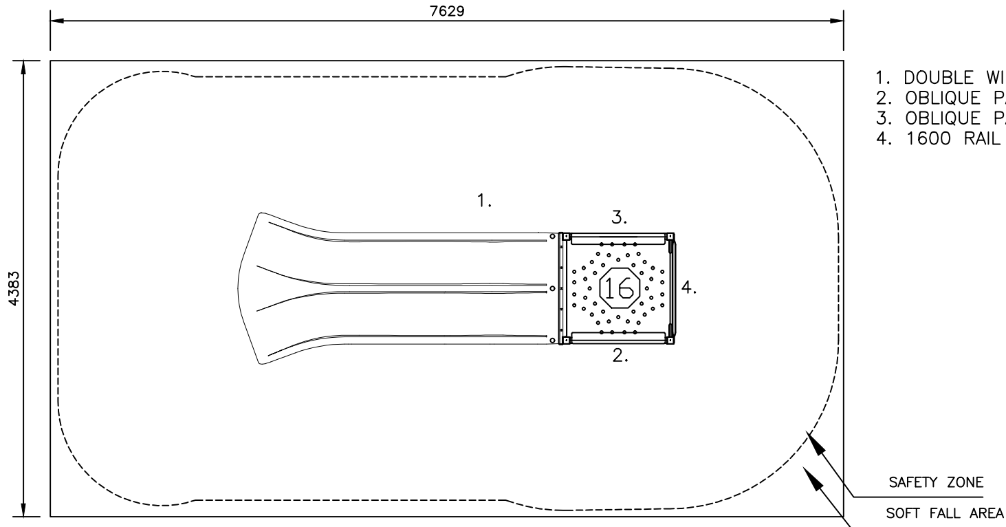
SLDP2017-1600 DOUBLE WIDE FREESTANDING SLIDE MAX FHF: 1.6M
